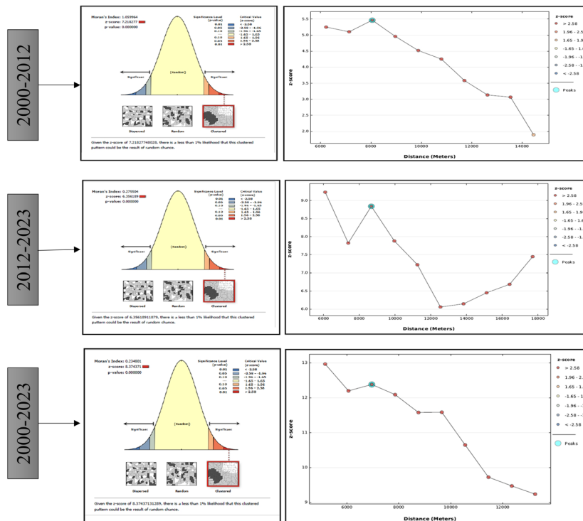
Fig. 4. Depiction of a significant pattern of Moran's I and the Distance band with the peak value in the three study periods
