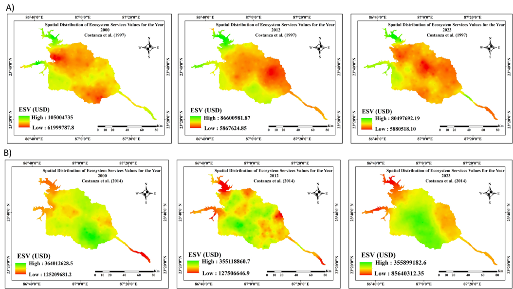
Fig. 3. Spatial Distribution of ecosystem services values A) as per Costanza et al. 1997 B) as per Costanza et al. 2014
