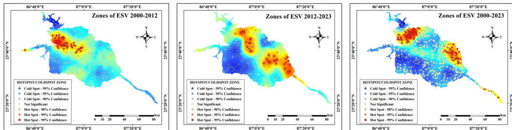
Fig. 5. The concentration zone of Hot spot and Cold Spot in ecosystem services values
