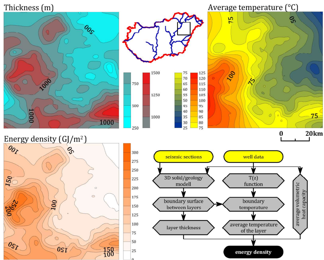
Fig. 1. Calculation of the theoretical geothermal potential of the Pannonian reservoirs in Hortobágy-Hajdúság-Nyírség study area (base maps, flow diagram and result map)
