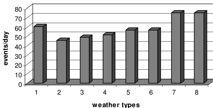
Fig. 3. Frequency of the patients registered with respiratory diseases in the eight weather types (clusters) received, summer – early autumn period (July 15 – October 15)
