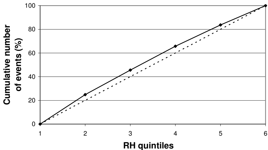
Fig. 1. Lorenz curve of relative humidity and the total patient number, summer – early autumn period (July 15 – October 15)
