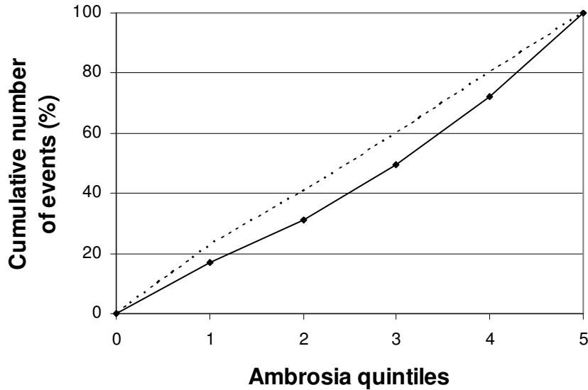
Fig. 2. Lorenz curve of Ambrosia pollen and the total patient number, summer – early autumn period (July 15 – October 15)
