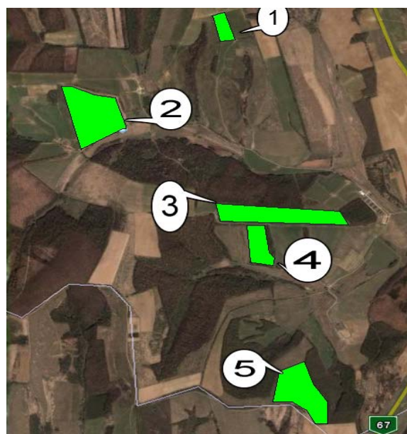
Figure 1: The examined grasslands at Bőszenfa
