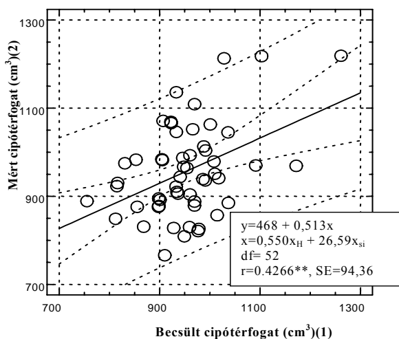
Figure 6: Regression between observed loaf volume and with QTS25 and MININFRA data estimated loaf volume (SE%=9,98) ( X_H Hardness; X_{si} MININFRA moisture gluten content) Estimated loaf volume (cm 3 )(1), Observed loaf volume (cm 3 )(2)
