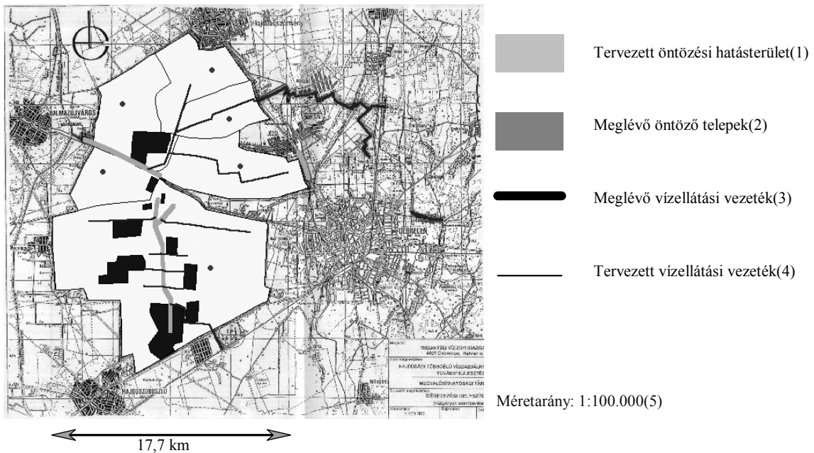
Figure 4: Digitised image of the area impounded on Hajdúsági Lőszhát (loess ridge) in respect of irrigation improvement The affected zone of planned irrigation(1), Present irrigation farms(2), Present water supply canal(3), Planned water supply canal(4), Scale: 1:100.000(5)
