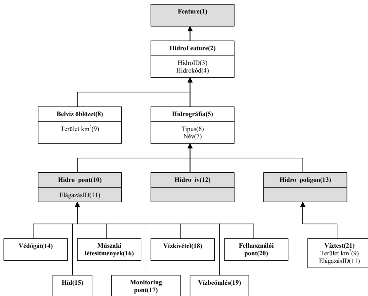
Figure 2: UML diagram of Hydrography component of a geodatabase
