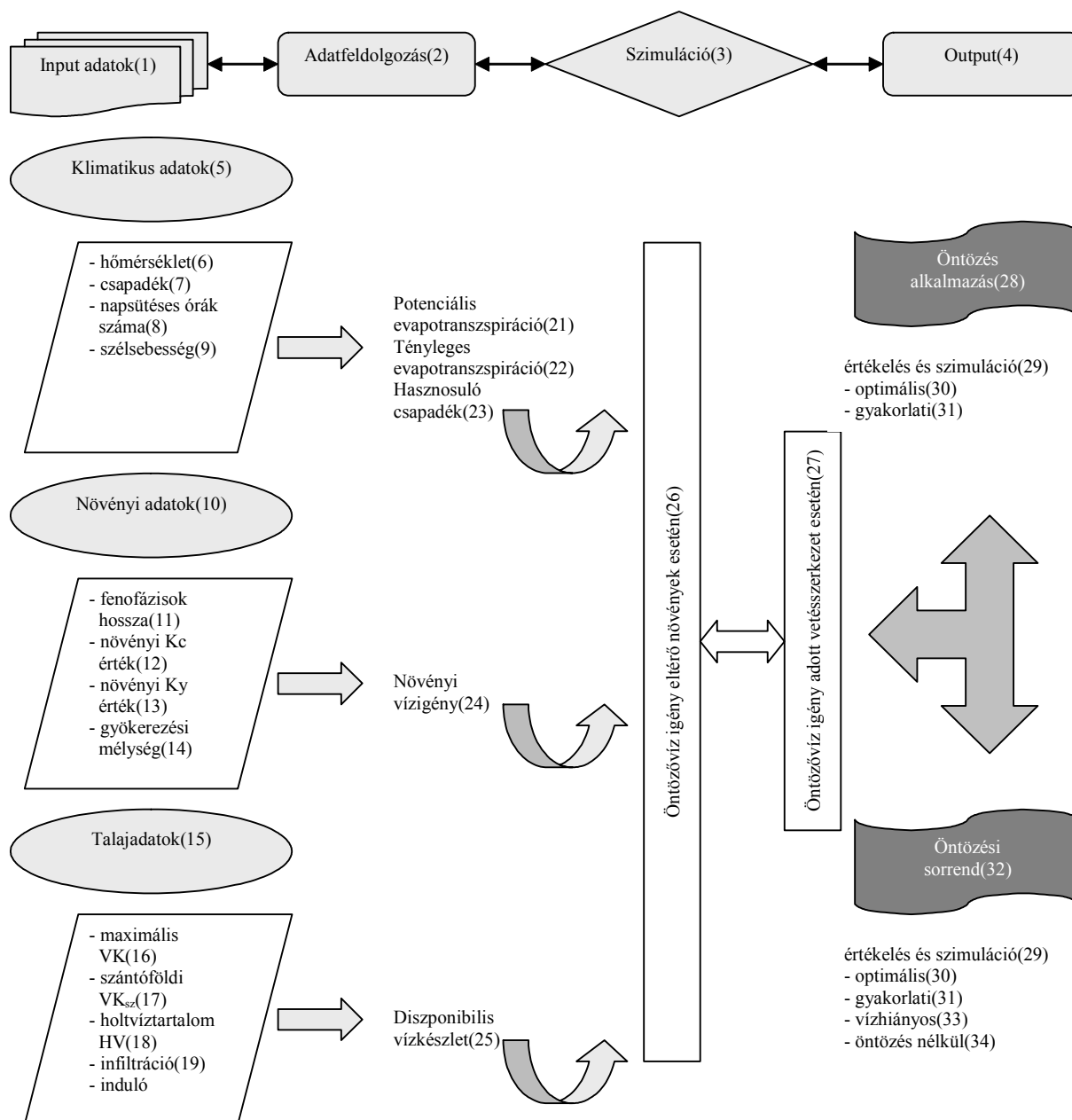
Figure 6: Logic model of CROPWAT-program
