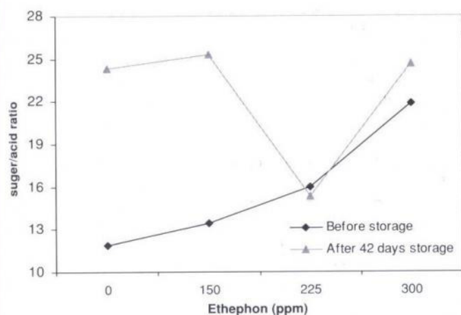
Figure 2. Effect of ethephon treatments (0 [control], 150, 225, 300 ppm) before storage and after storage on sugar:acid ratio of sour cherry fruits under modified atmosphere packaging and 0 °C conditions
