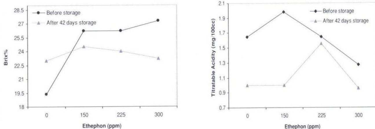
Figure 1. Effect of ethephon treatments (0 [control], 150, 225, 300 ppm) before storage and after storage on chemical attribute of sour cherry fruits in modified atmosphere packaging and 0 °C conditions
