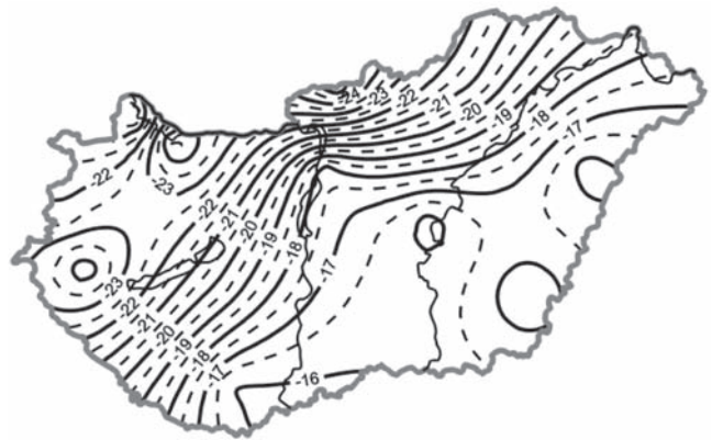
Figure 1 – The spatial distribution of absolute temperature minima in spring measured at 16 stations over a period of 1951–2010
