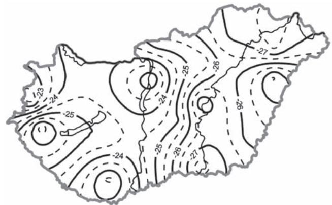
Figure 2 – The absolute minimum temperatures during winter according to data raised at 16 stations over a period of 1951–2010
