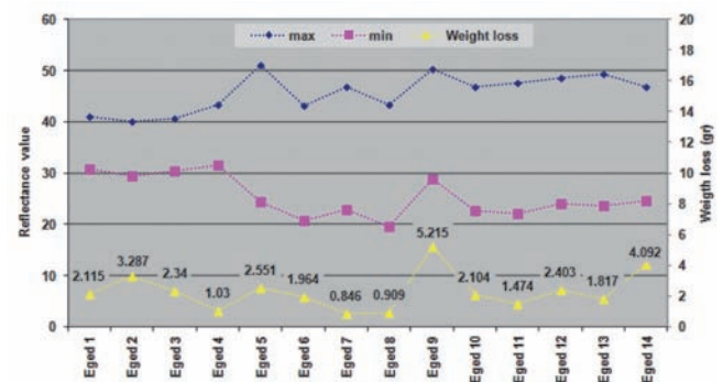
Figure 7: Maximum and minimum reflectance value of green leaves within 900–970 nm wavelength intervals, and the values of the total weight loss of leaves originated from water content (from 495 m to 310 m above see level)
