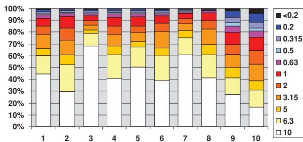
Figure 5: Grain size distribution of soil samples in 0–10 cm depth, from 495 m to 310 m above see level
